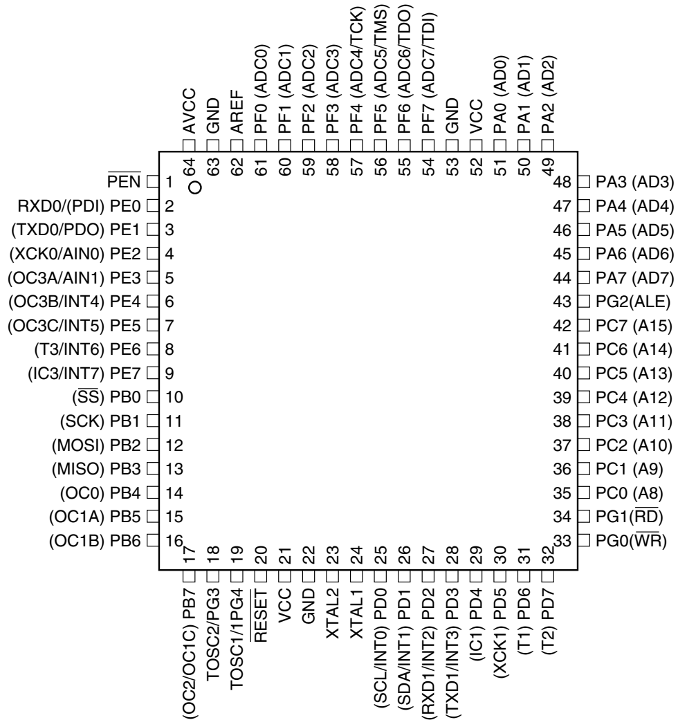
Figure 1. Pinout ATmega128
