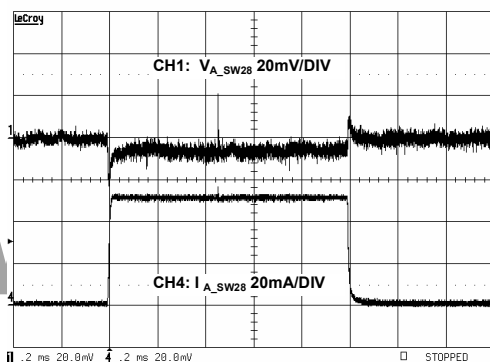
V A_SW28 Load Transient
