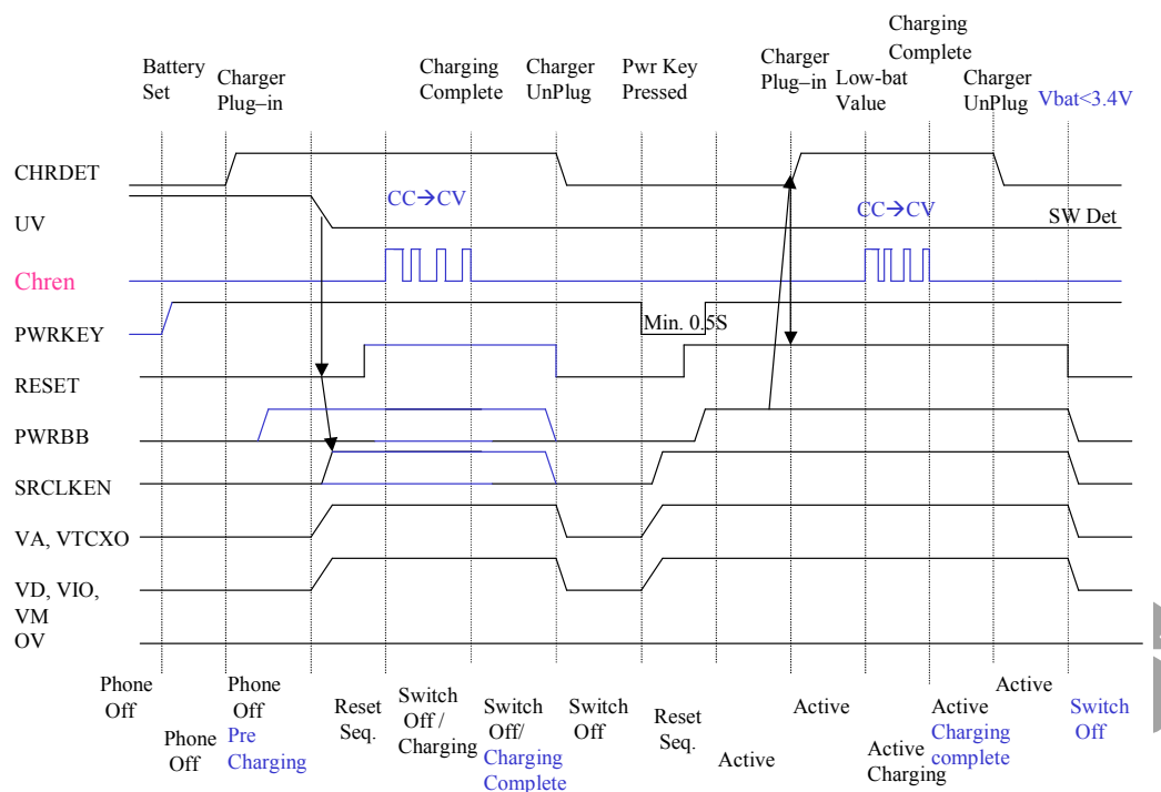
Figure 7: Charger State Timing
