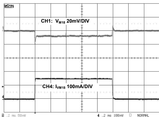
V_{\text{M18}} Load Transient
