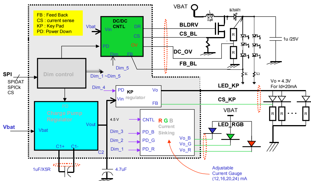
Figure 13: LED Driver Block Diagram
