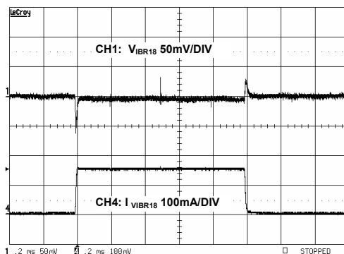
V IBR18 Load Transient
