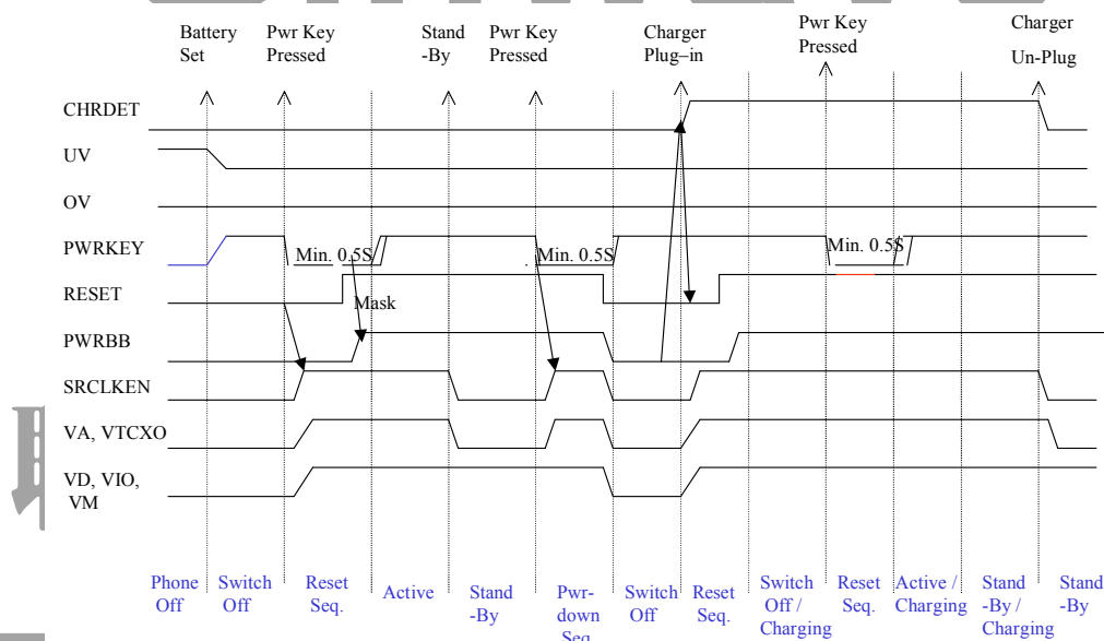
Figure 5: Power Key State Timing
