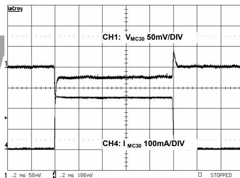
V_{MC30} Load Transient
