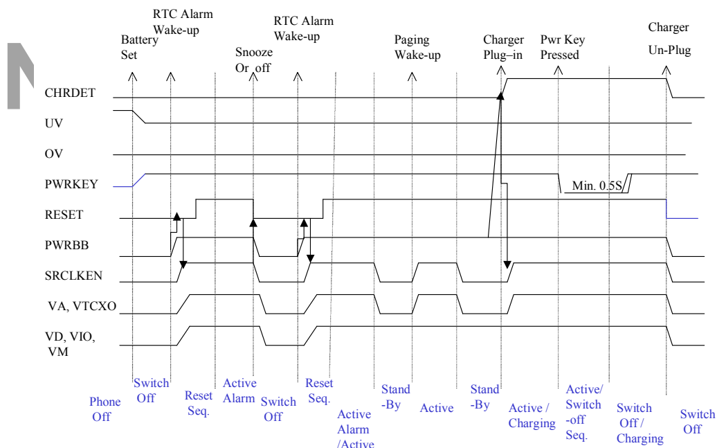
Figure 6: State Timing for Wake-up, Paging and Standby
