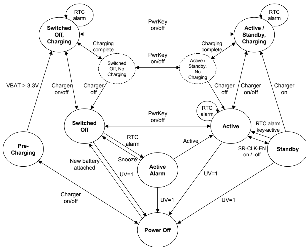
Figure 3: Power Management State Diagram
