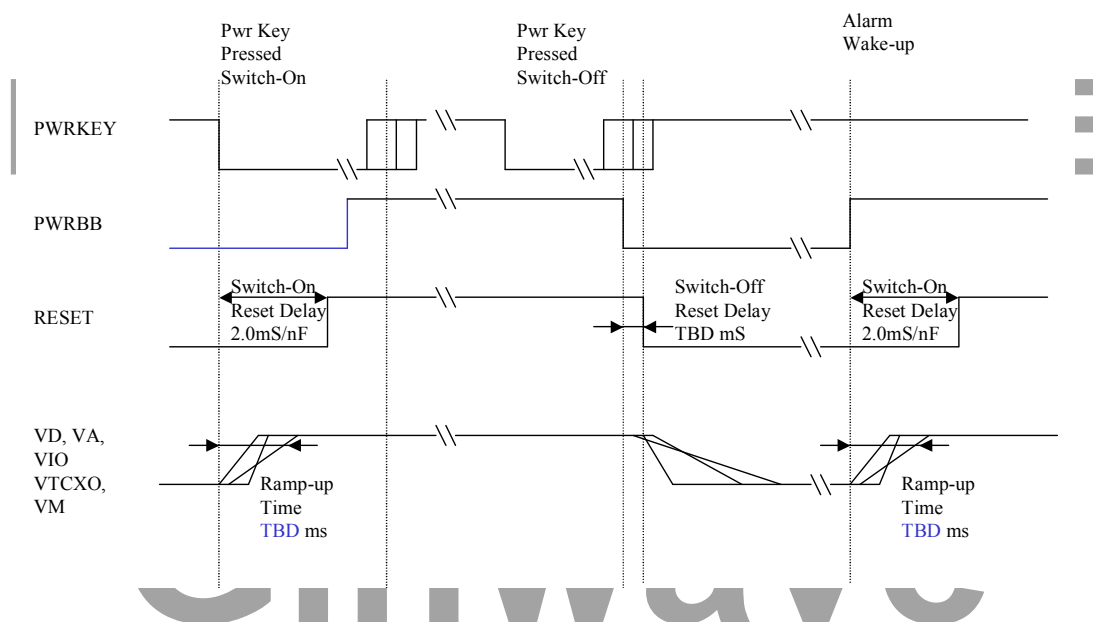
Figure 8: Reset Timing
