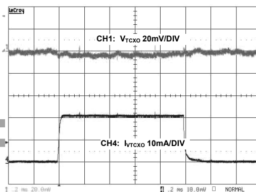
V_{\text{TCXO}} Load Transient
