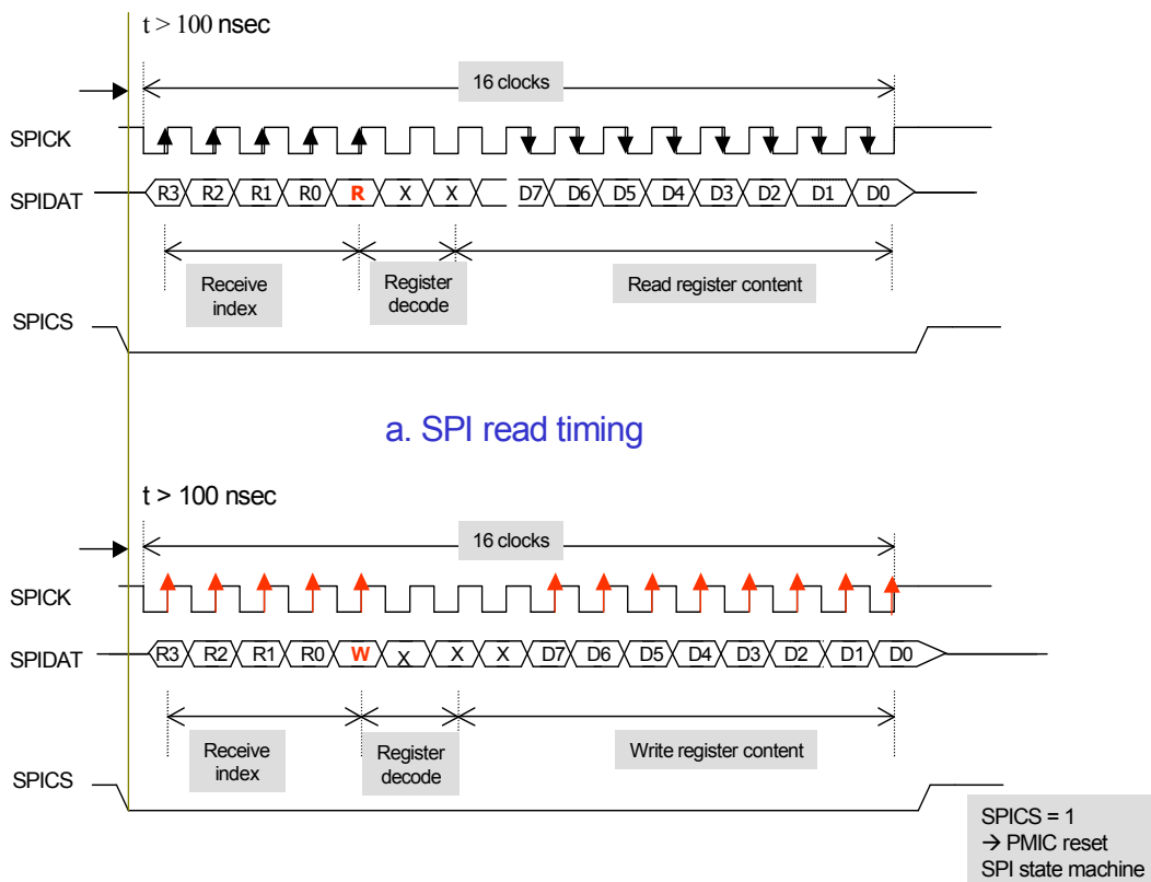
b. SPI write timing
