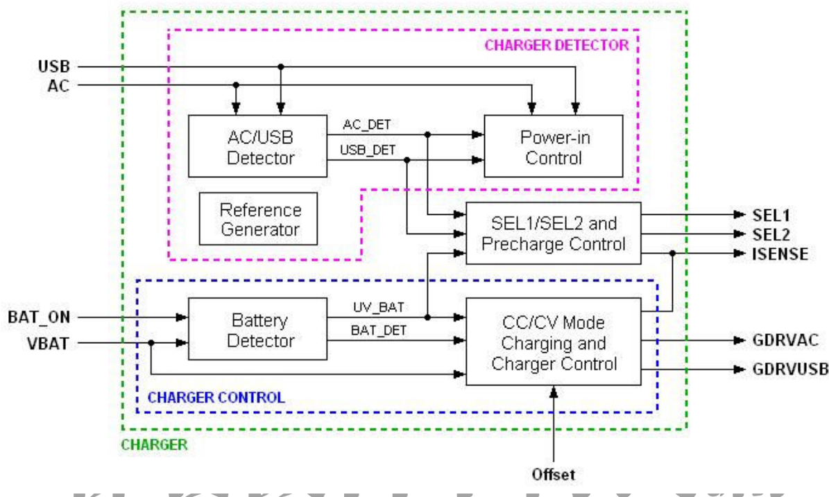
Figure 10: PMIC Charger Block Diagrams
