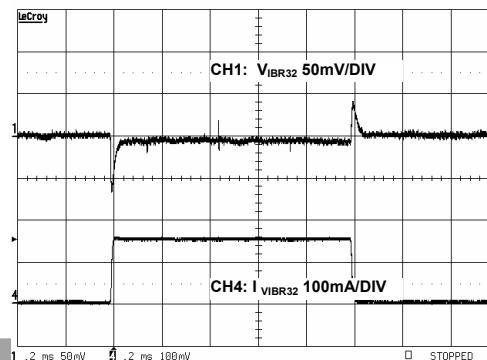
V IBR32 Load Transient
