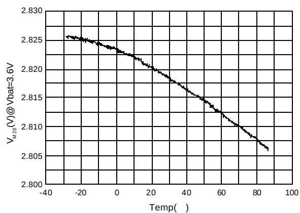
V_{M28} vs. Temp
