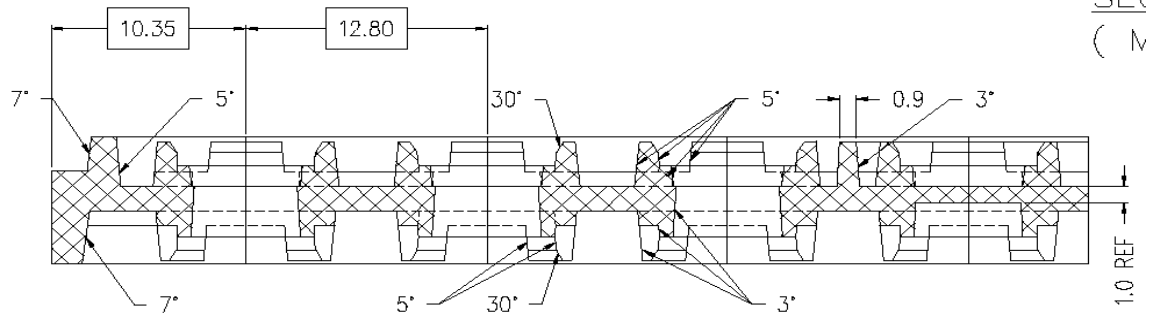
SECTION B-B ( M 5:1 )
