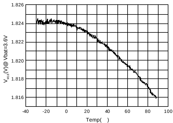
V_{M18} vs. Temp
