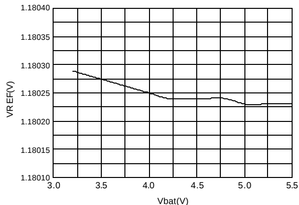
V_{REF} vs. Vbat
