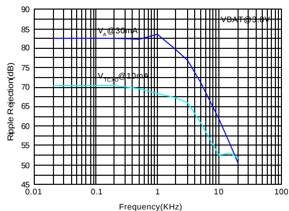
V_A & V_{TCXO} Ripple Rejection vs. Frequency
